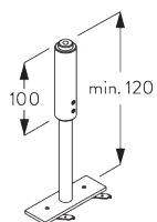
SG 6105 Suspension
