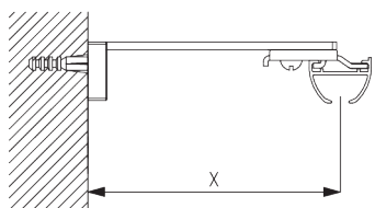
Square Smart Fix SG 11210 - SG 11215 et support SG 3832:
