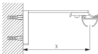
Smart Fix SG 11200 - SG 11205 et support SG 3832:
