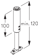
SG 6190 Suspension
